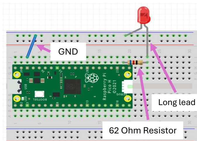
Example Single LED circuit
