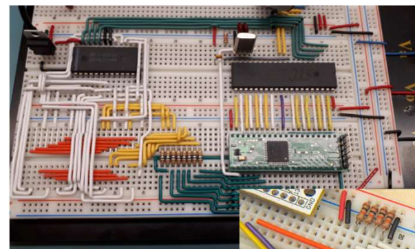
Examples of good breadboard technique
