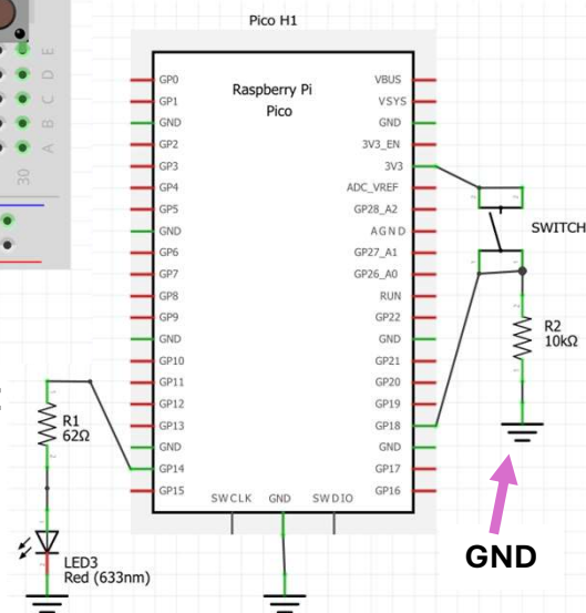
Example pushbutton & LED circuit (GP pins are arbitrary)
