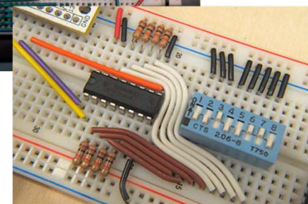
Examples of good breadboard technique
